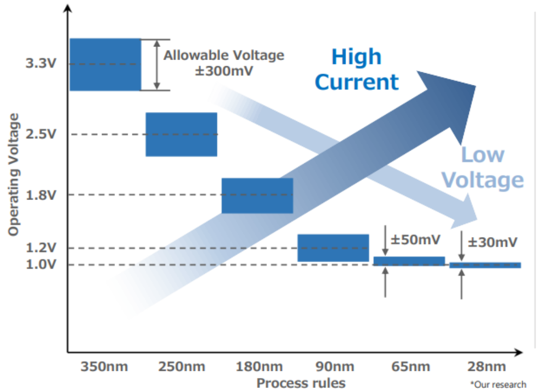
Figure 1: The transition of semiconductor power supply voltages. (Source: TAIYO YUDEN)
